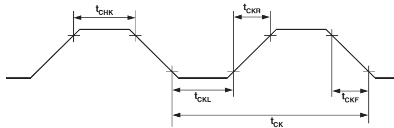
Figure 67. XTAL1 Input
