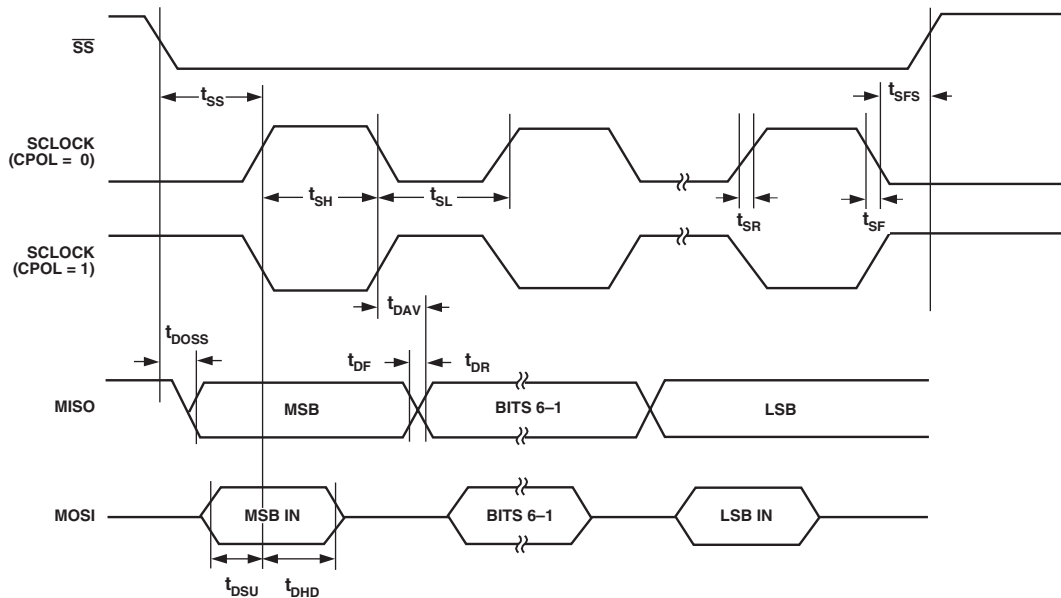
Figure 76. SPI Slave Mode Timing (CPHA = 0)
