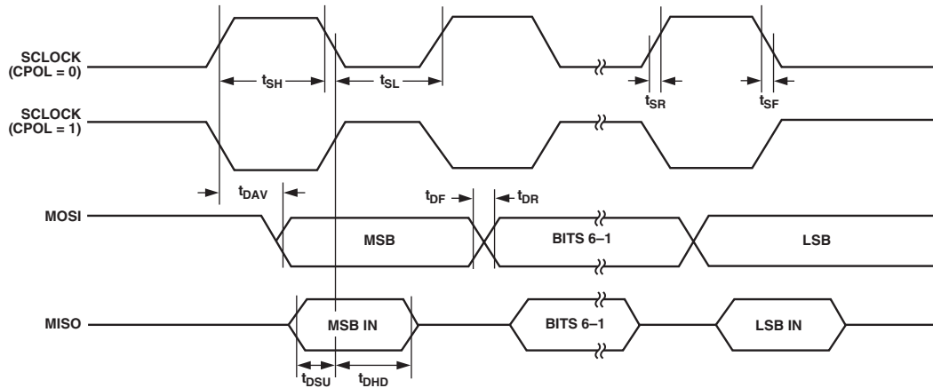
Figure 74. SPI Master Mode Timing (CPHA = 0)
