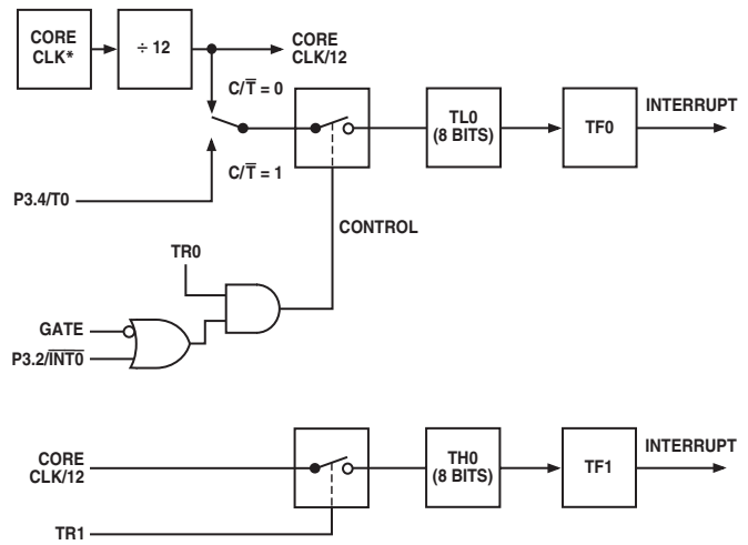
Figure 51. Timer/Counter 0, Mode 3
