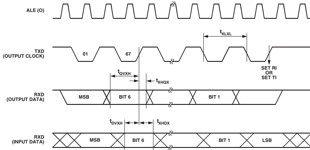
Figure 72. UART Timing in Shift Register Mode
