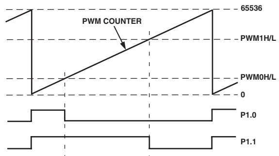
Figure 29. PWM Mode 3
