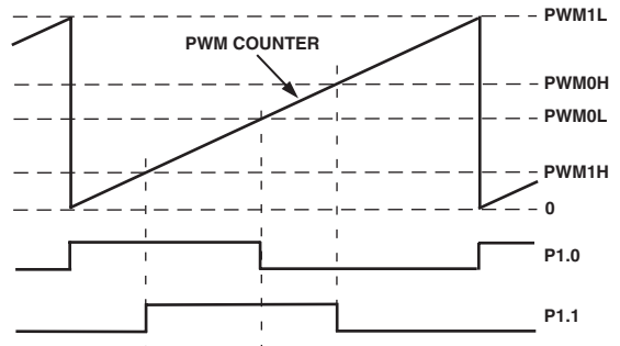
Figure 28. PWM Mode 2
