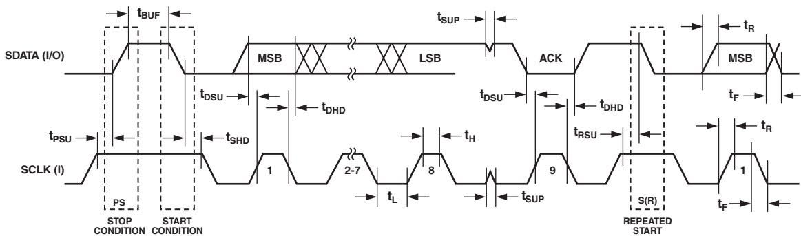
Figure 77. I 2 C Compatible Interface Timing
