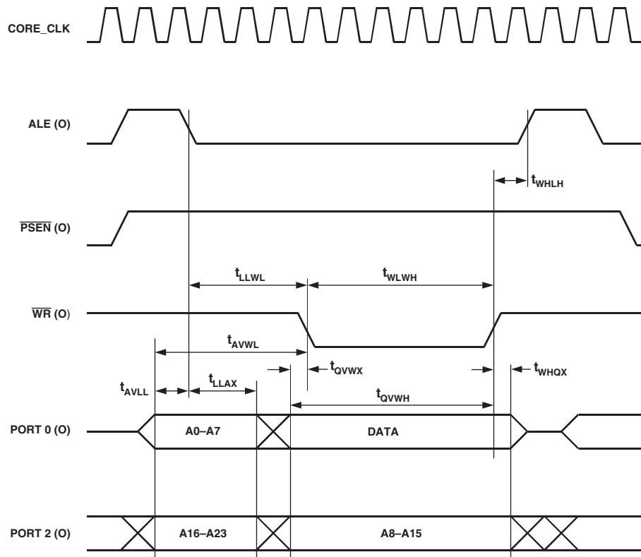
Figure 71. External Data Memory Write Cycle
