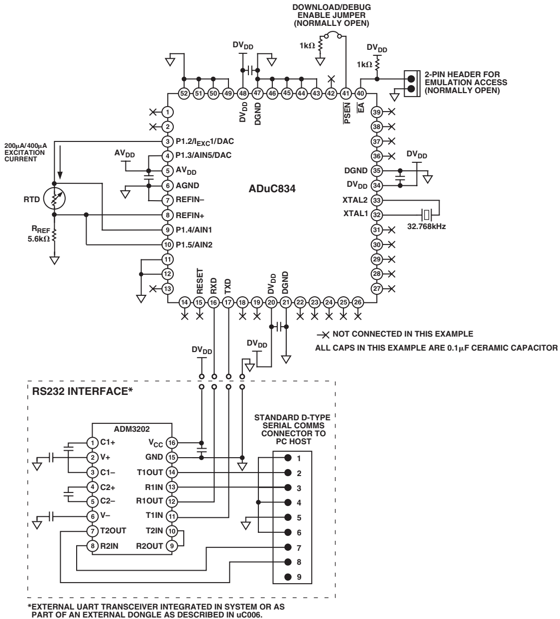
Figure 66. Typical System Configuration
