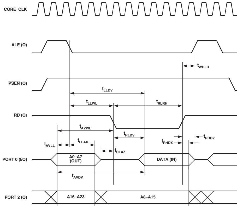
Figure 70. External Data Memory Read Cycle
