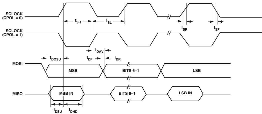
Figure 73. SPI Master Mode Timing (CPHA = 1)
