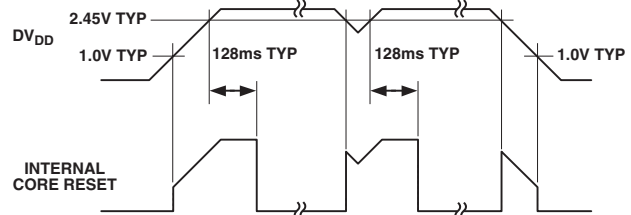
Figure 63. ADuC834 Internal Power-on-Reset operation
