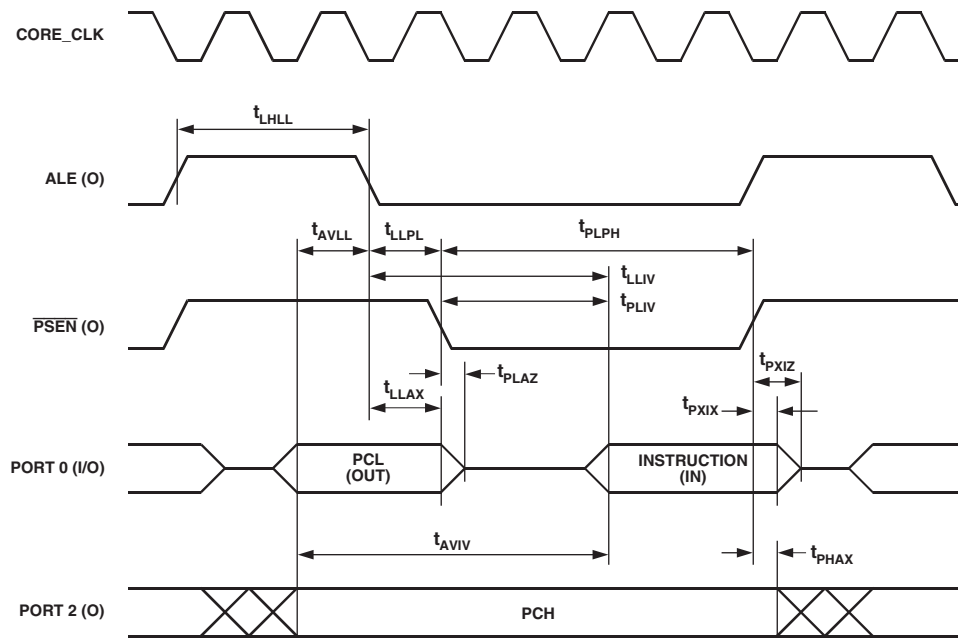
Figure 69. External Program Memory Read Cycle
