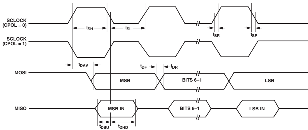
Figure 75. SPI Slave Mode Timing (CPHA = 1)
