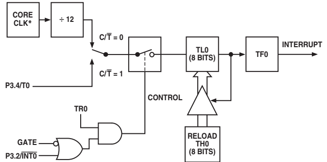
Figure 50. Timer/Counter 0, Mode 2
